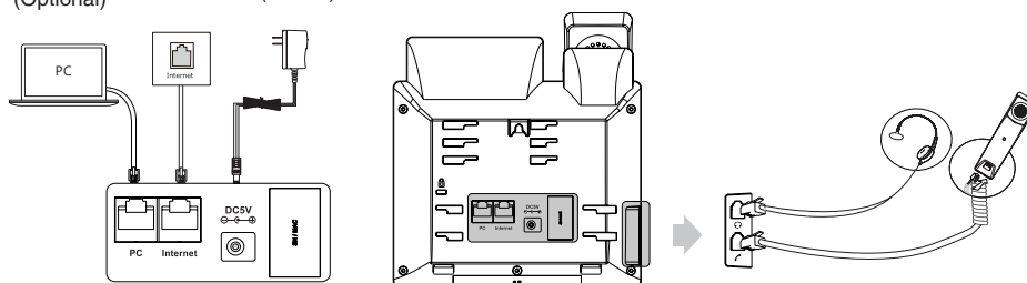
Power Adapter (DC 5V)
